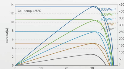
I-V/P-V Curve at Different Irradiation (420W)
